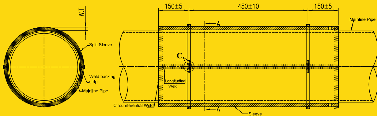
basic drawing reinforcement sleeve
